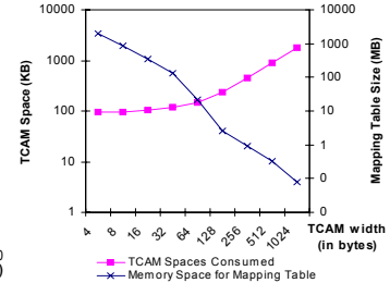
Figure 7. Impact of TCAM Width
