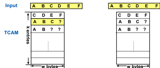
3.a First Position 3.b Second Position Figure 3. Scanning Process.
