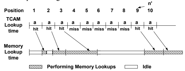
Figure 5. Memory Lookup Process.
